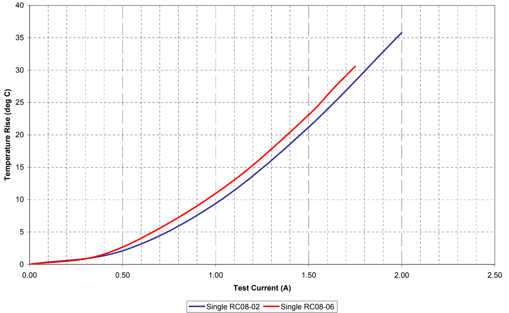
Single Pin Energized: RC08-0X with CE08LG03
