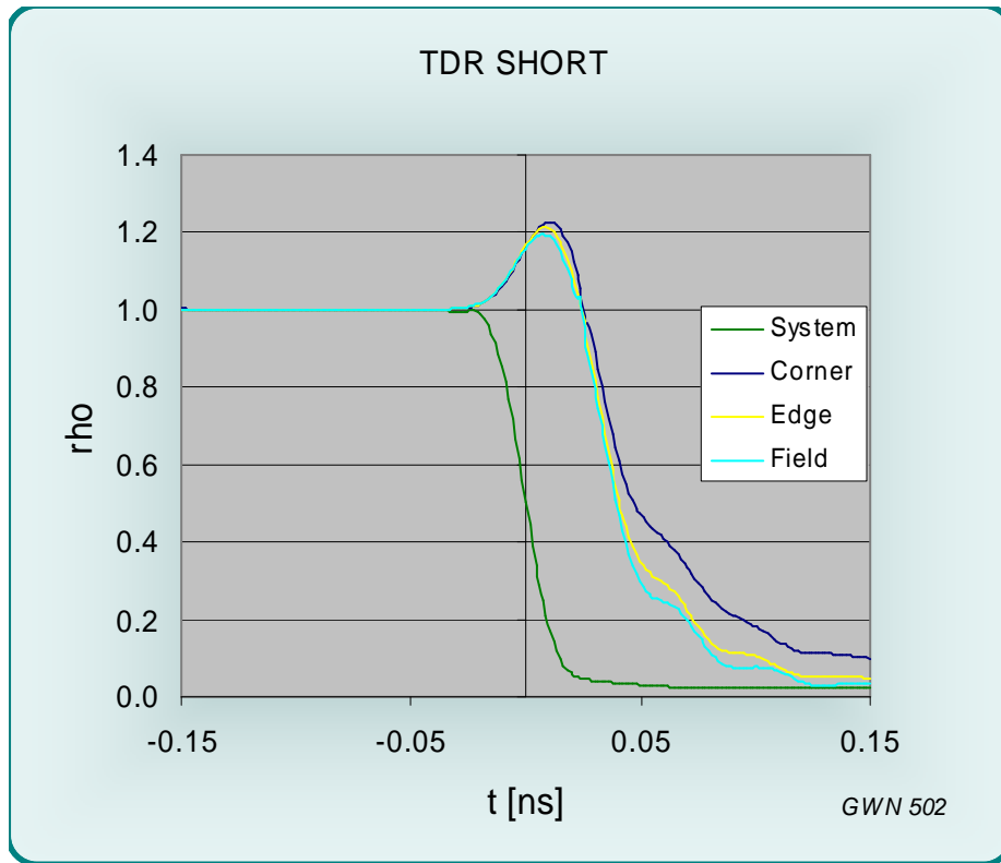
Figure 6 TDR signal from a SHORT circuited SK05-0097T socket
