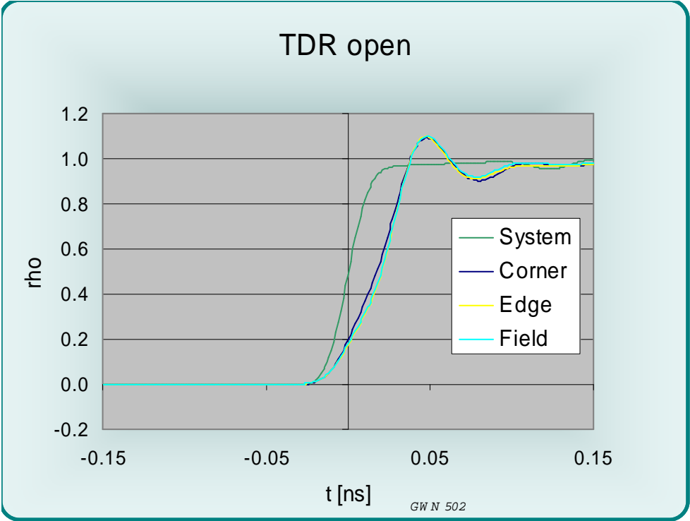
Figure 5 TDR signal from an OPEN circuited SK05-0097T socket
