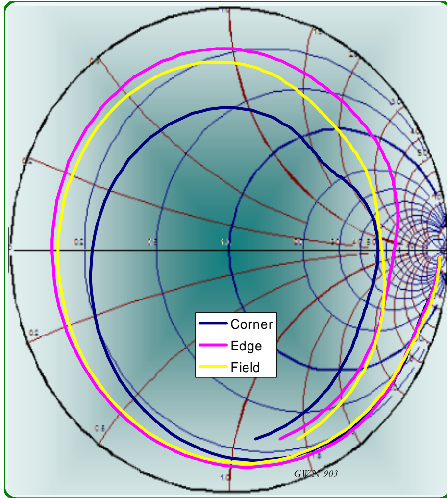
Figure 12 Reflections from the open circuited SK05-0097T socket
