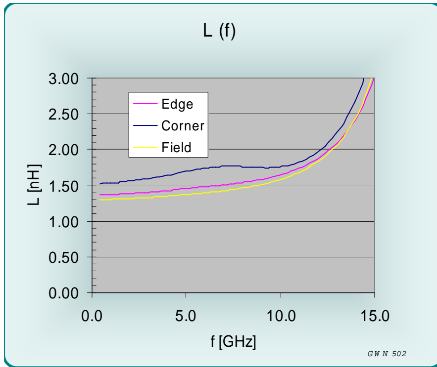
Figure 15 L(f) for the SK05-0097T socket
