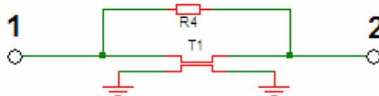
Figure 31 Transmission line model for the SK05-0097T socket
