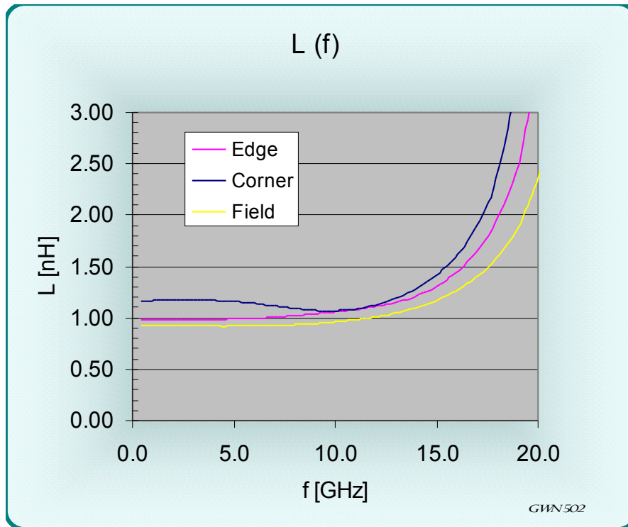
Figure 15 L(f) for the SK05-0126T socket
