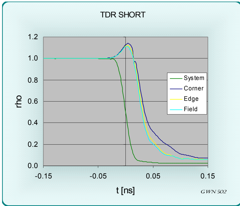
Figure 6 TDR signal from a SHORT circuited SK05-0126T socket
