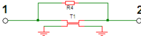
Figure 31 Transmission line model for the SK05-0126T socket
