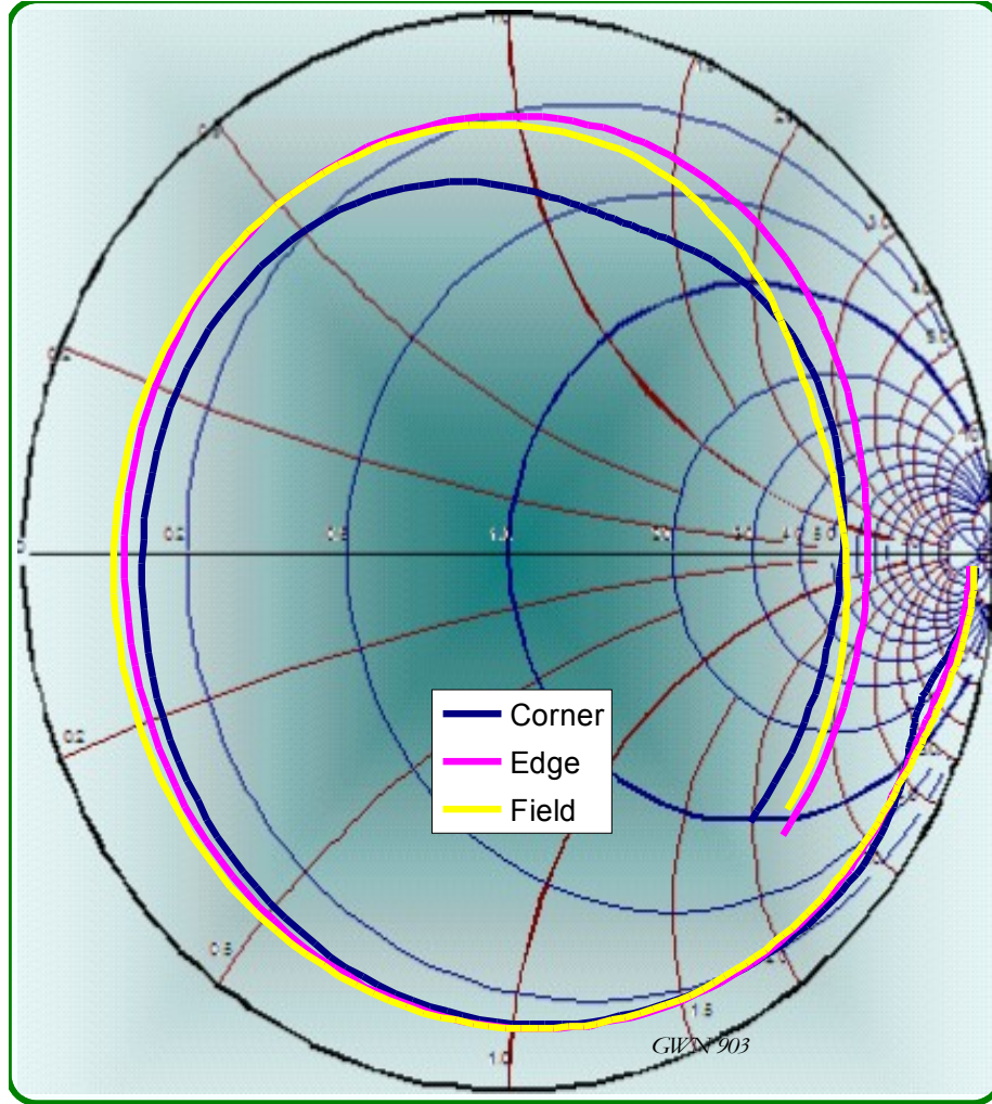
Figure 12 Reflections from the open circuited SK05-0126T socket
