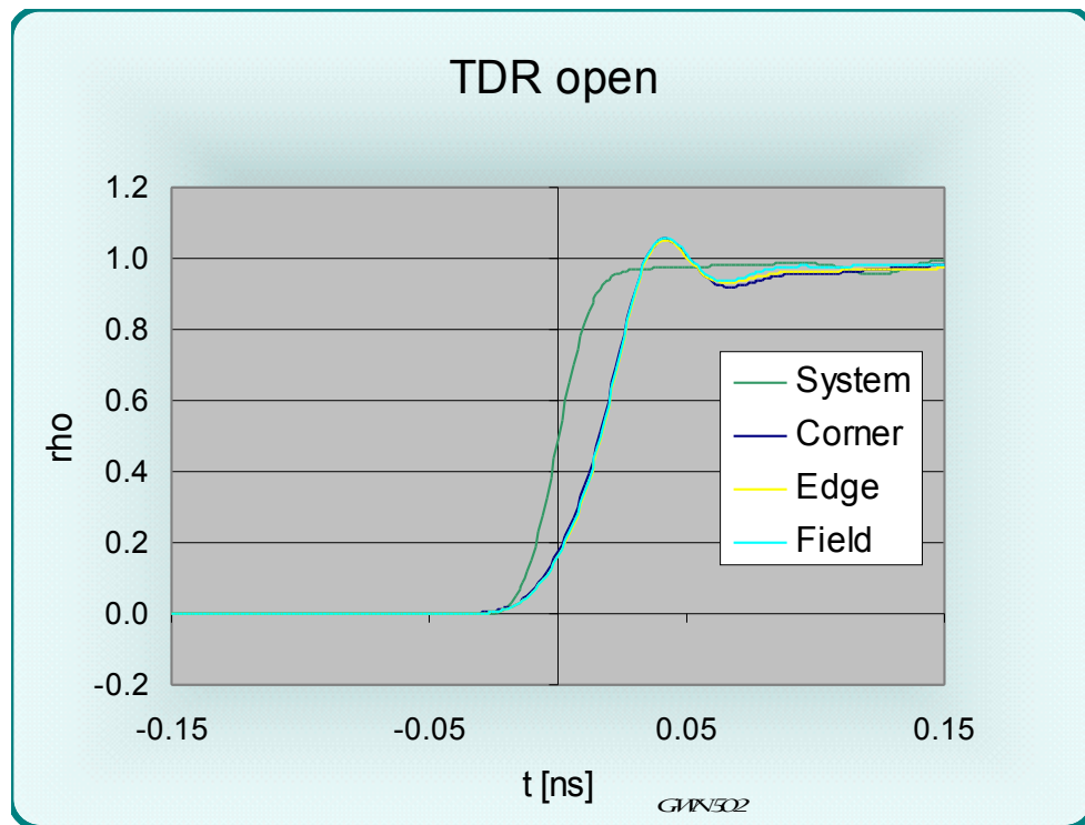
Figure 5 TDR signal from an OPEN circuited SK05-0126T socket
