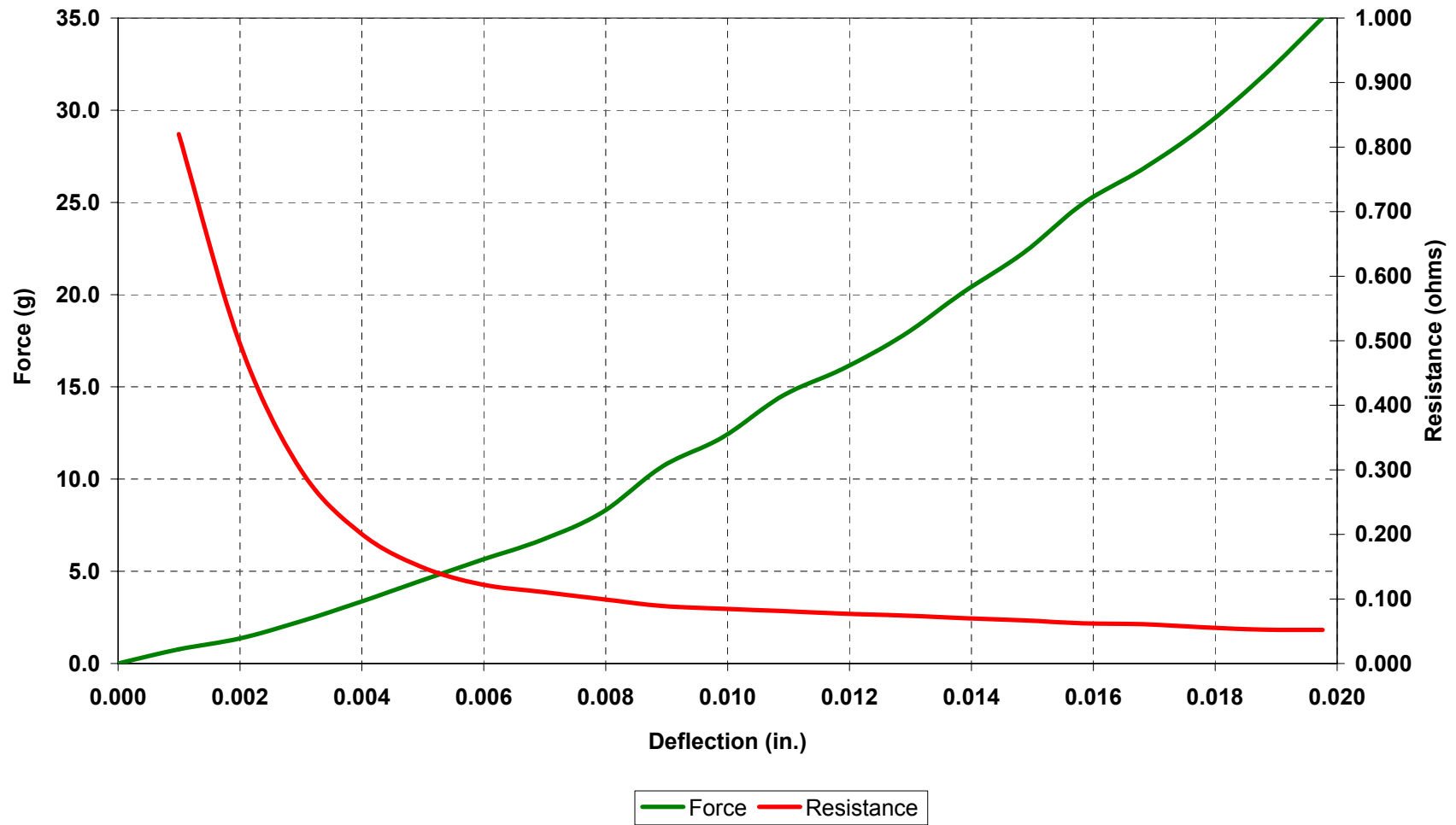
RC10-12 with Reduced Crown Force-Deflection-Resistance
