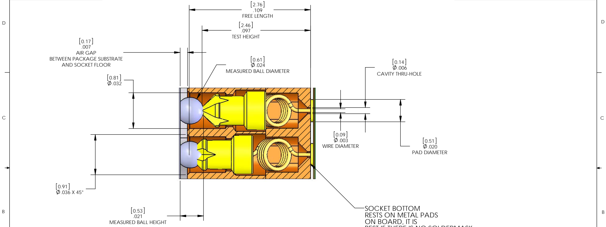
DETAIL B SCALE 30 : 1
