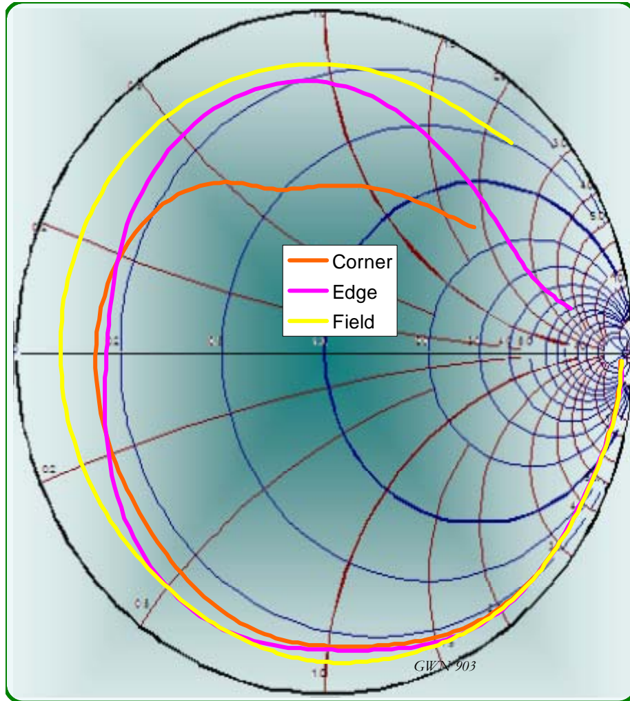
Figure 12 Reflections from the open circuited CR08-062 test socket
