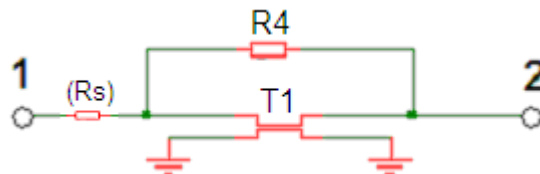
Figure 31 Transmission line model for the CR08-062 test socket
