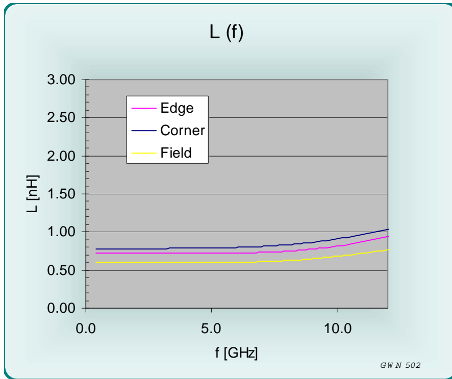
Figure 15 L(f) for the CR08-062 test socket
