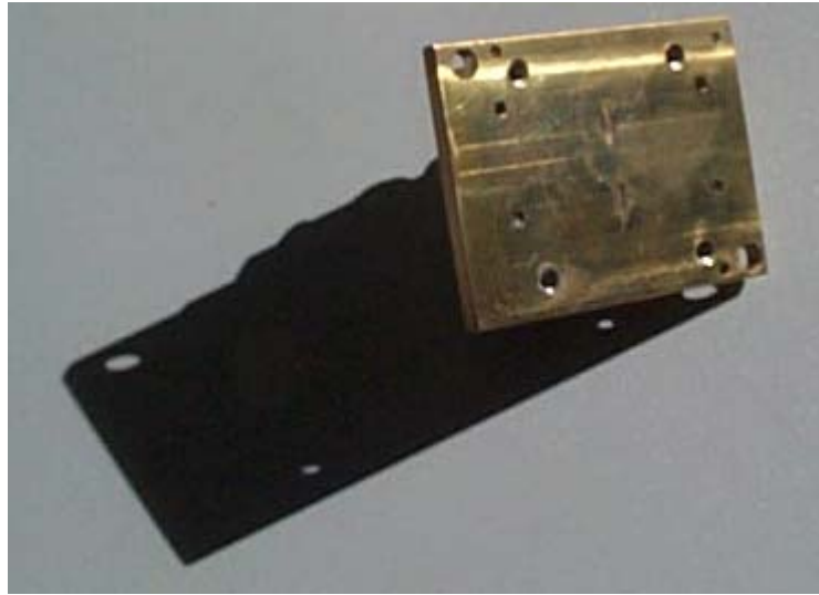
Figure 1 CR08-062 test socket base plate example
