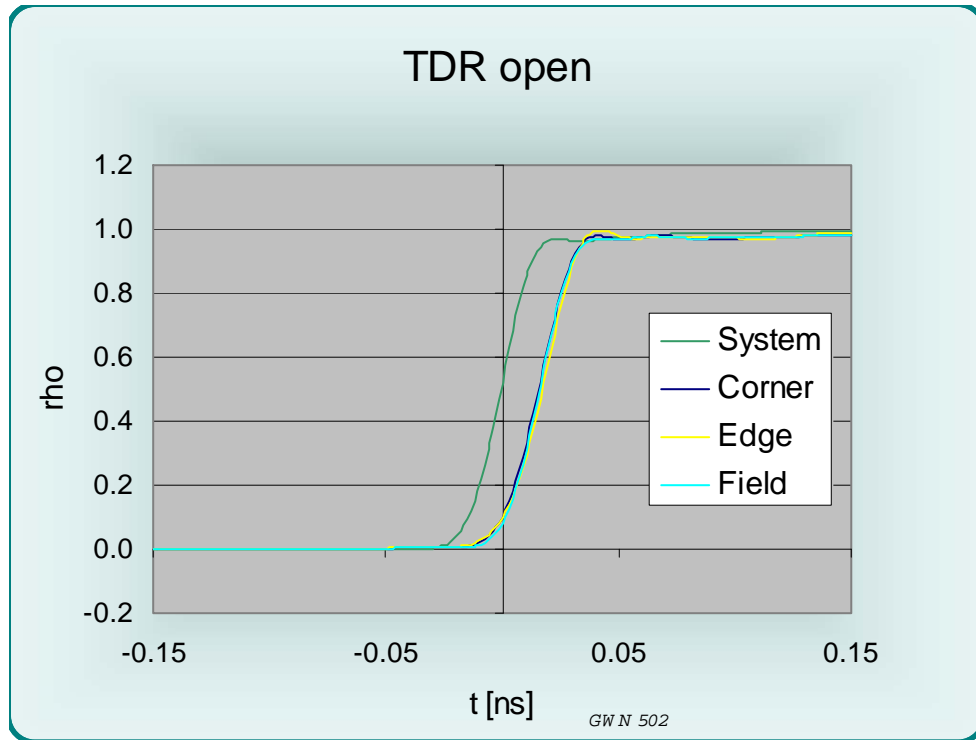
Figure 5 TDR signal from an OPEN circuited CR08-062 test socket
