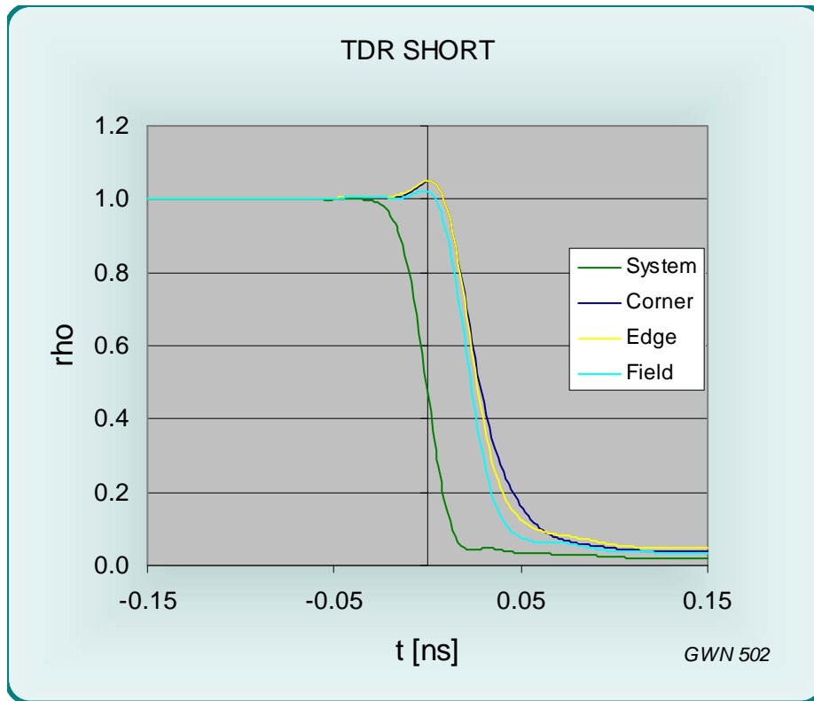
Figure 6 TDR signal from a SHORT circuited CR08-062 test socket
