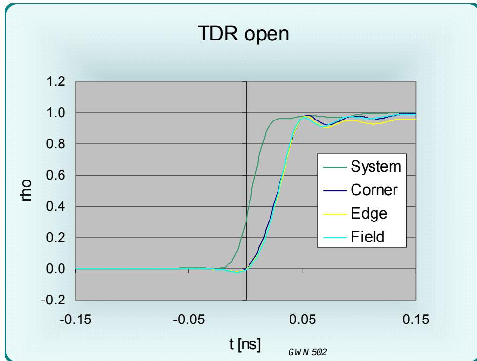
Figure 5 TDR signal from an OPEN circuited CR08-01 test socket
