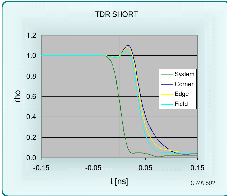
Figure 6 TDR signal from a SHORT circuited CR08-01 test socket
