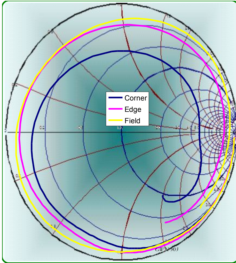
Figure 12 Reflections from the open circuited CR08-01 test socket
