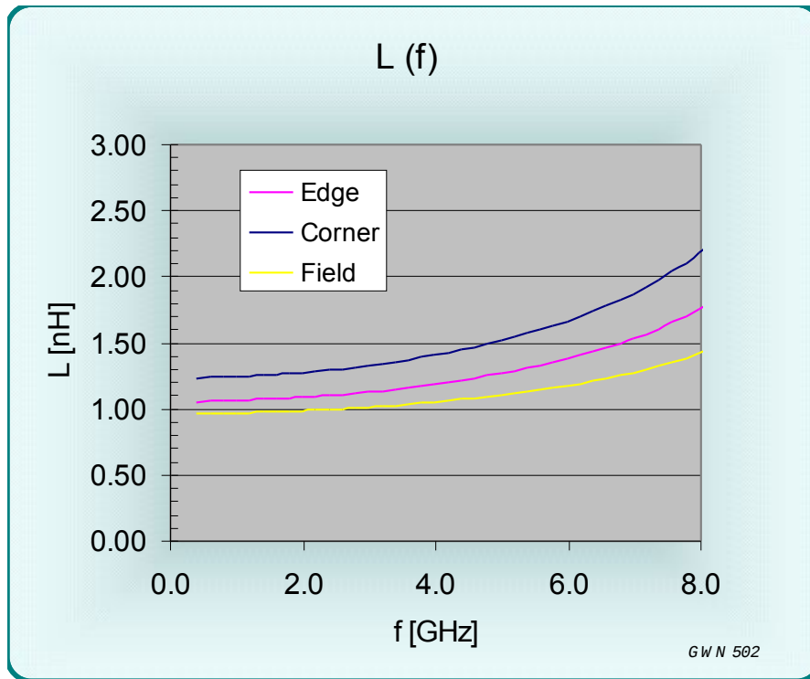
Figure 15 L(f) for the CR08-01 test socket
