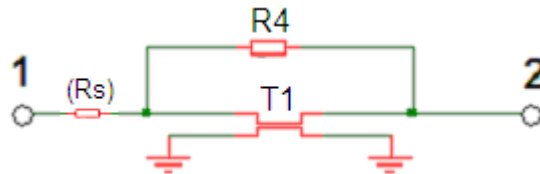
Figure 31 Transmission line model for the CR08-01 test socket
